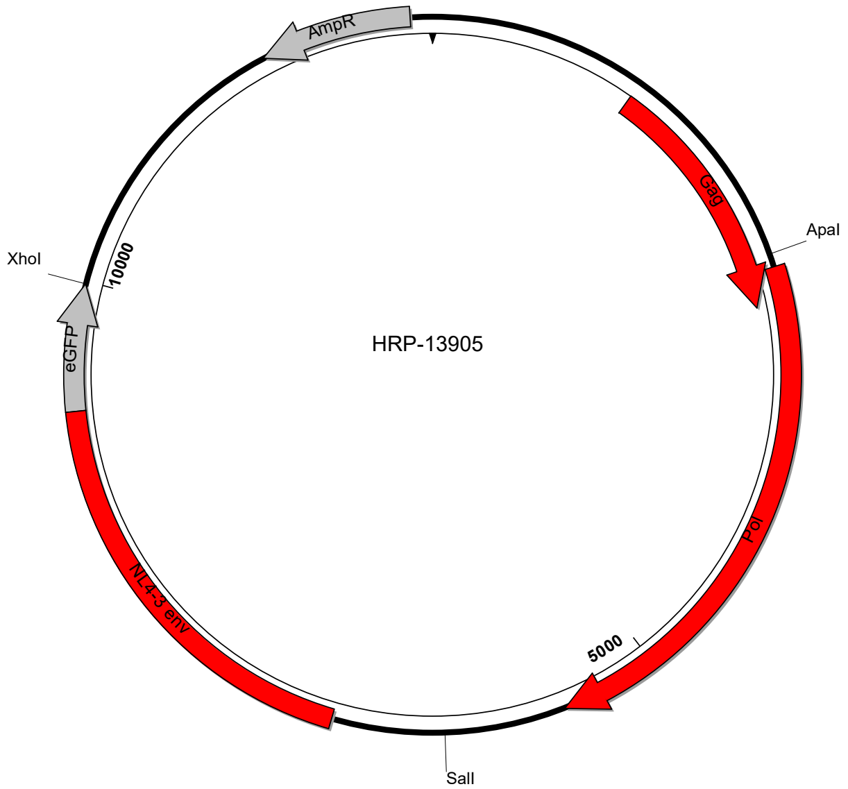
Figure 2: Plasmid Map of HRP-13905
